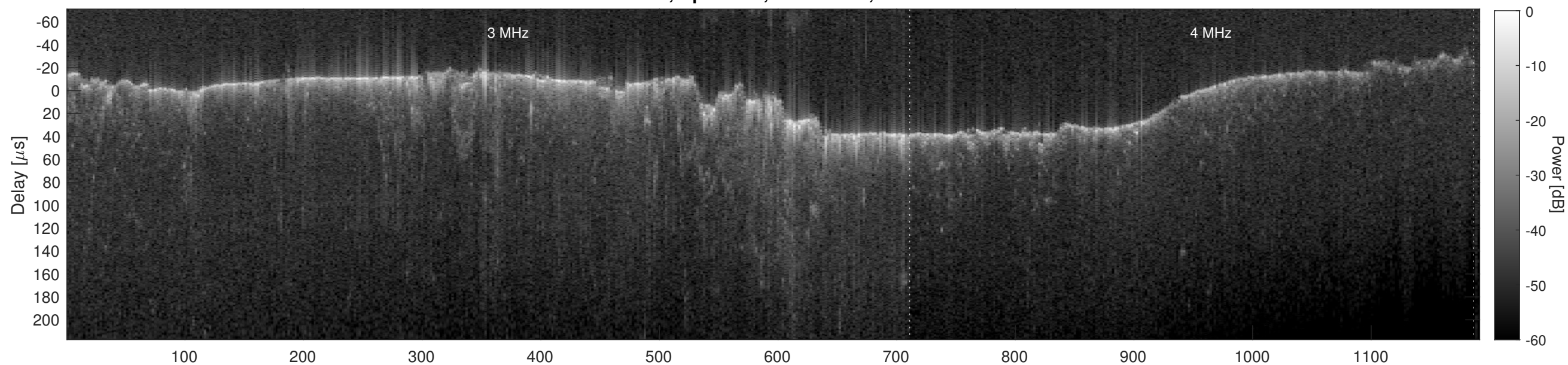
Orbit 7032, Cluttergram
