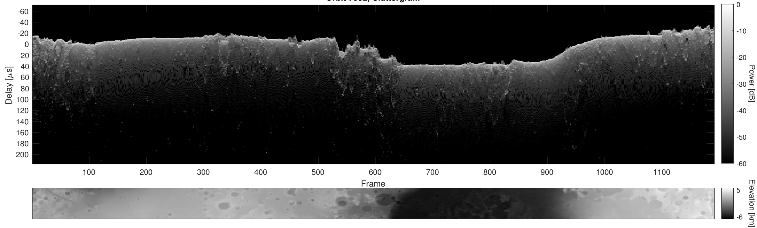
Orbit 7032, Cluttergram
