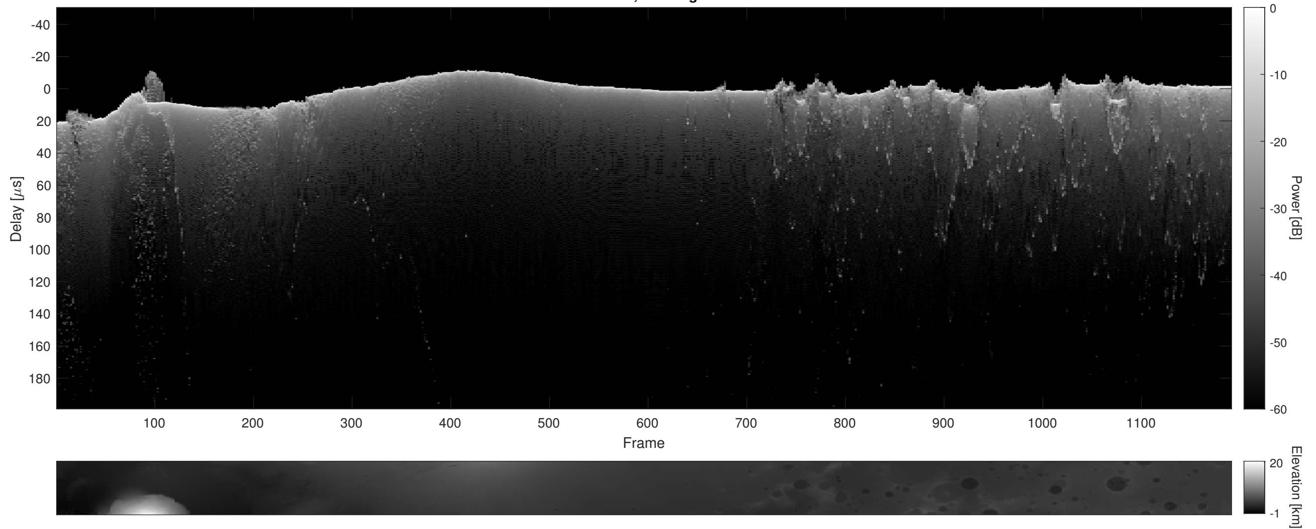
Orbit 7034, Cluttergram
