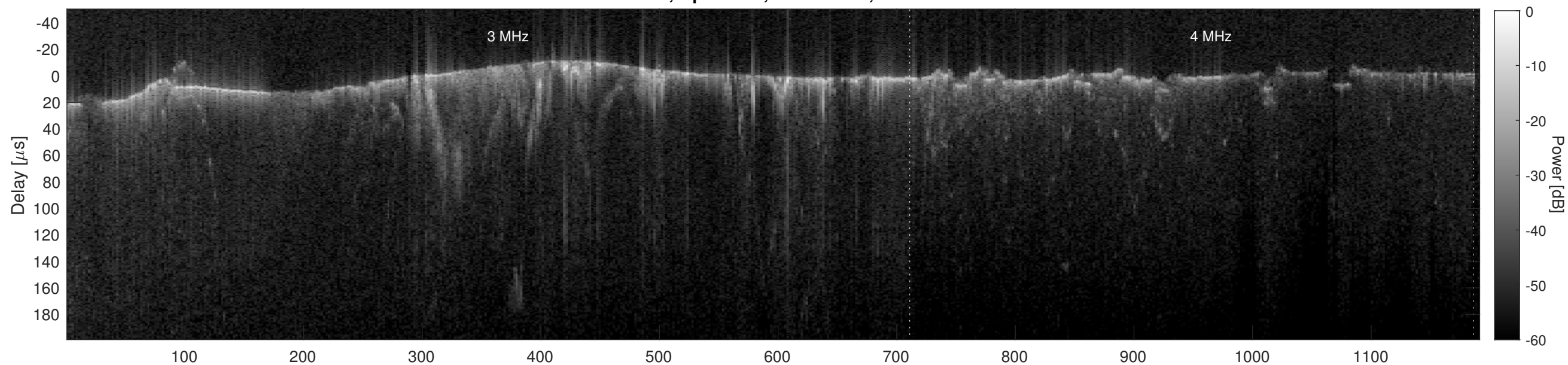
Orbit 7034, Cluttergram
