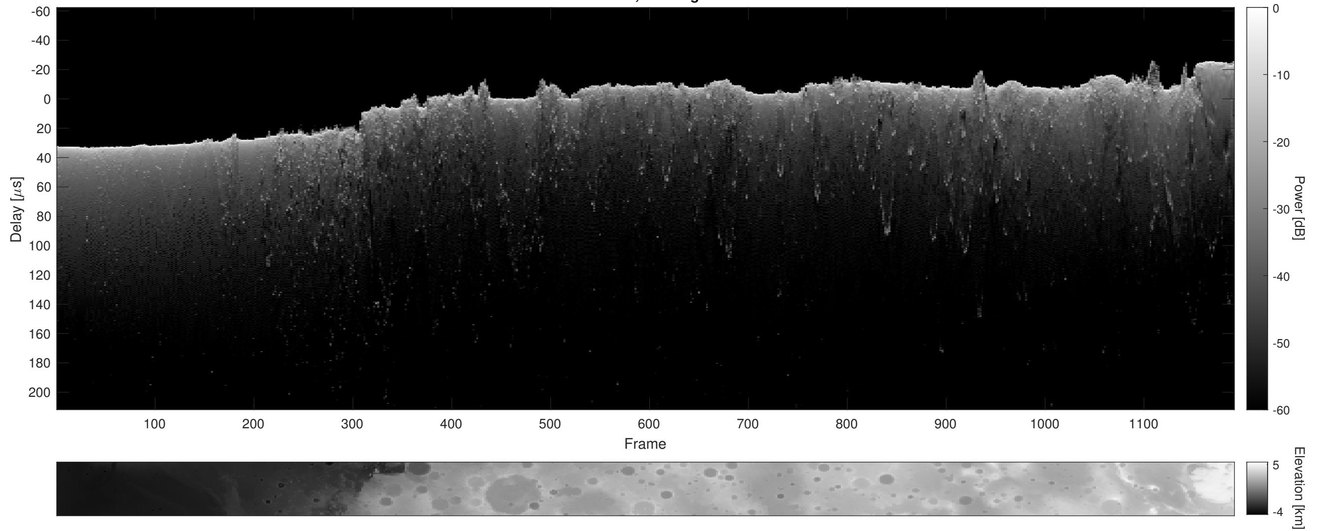
Orbit 7035, Cluttergram
