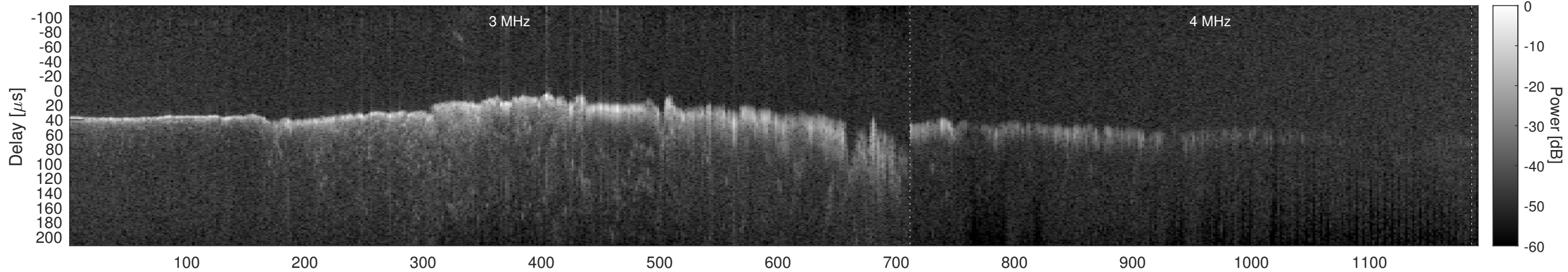
Orbit 7035, Window, Channel 2, Chapman
