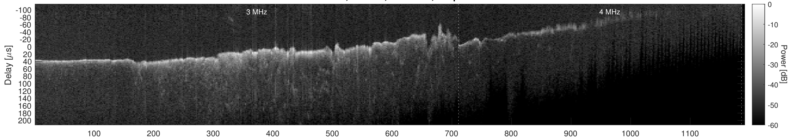
Orbit 7035, Window, Channel 2, Optimized
