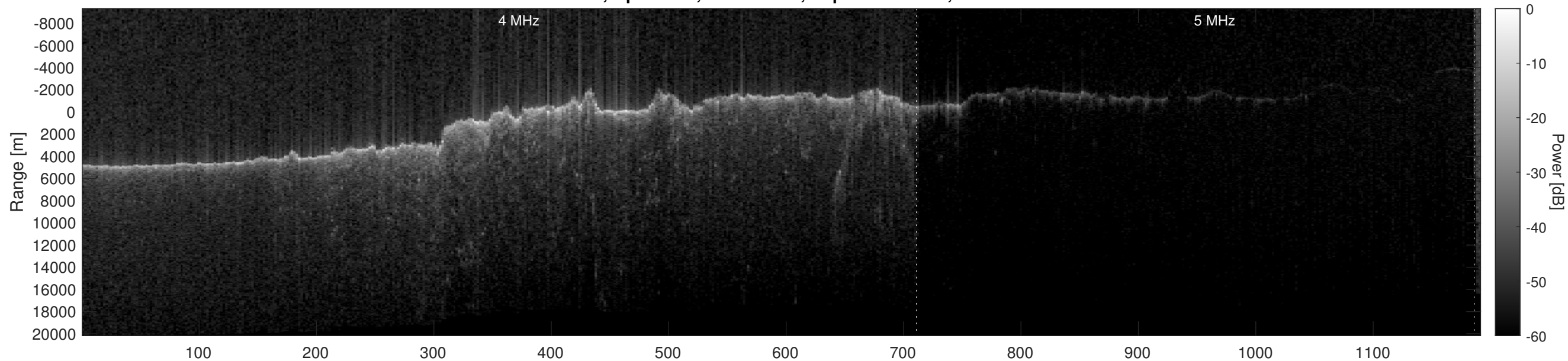
Orbit 7035, Optimized, No Window, Depth-Corrected, Channel 2
