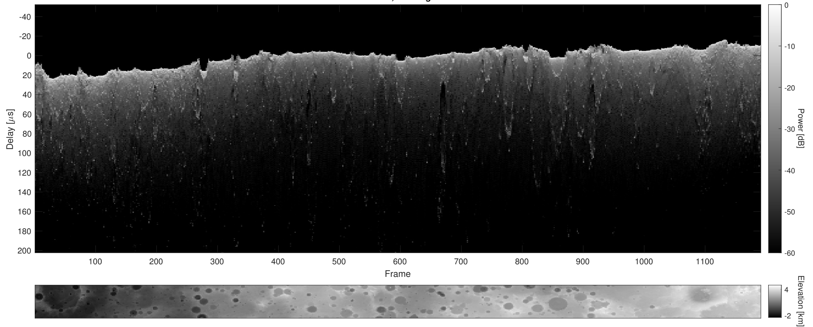
Orbit 7036, Cluttergram
