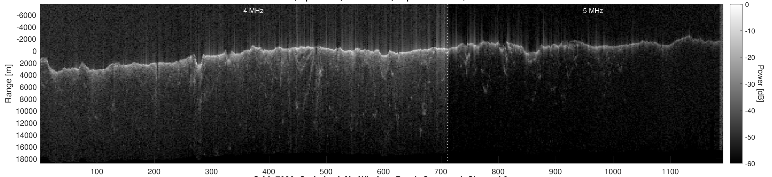
Orbit 7036, Optimized, No Window, Depth-Corrected, Channel 2
