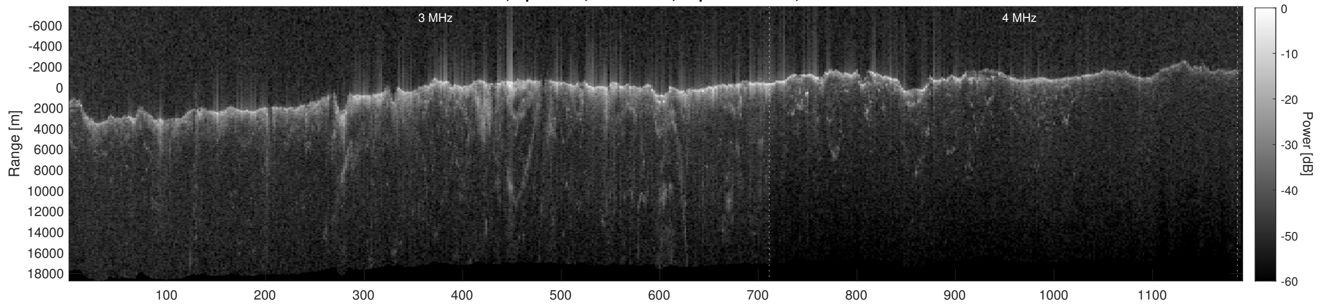
Orbit 7036, Depth-Corrected Cluttergram
