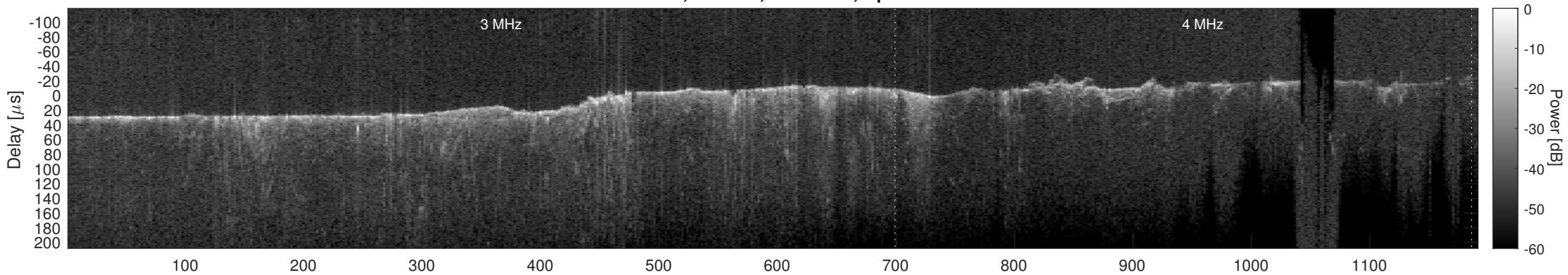
Orbit 7038, Cluttergram
