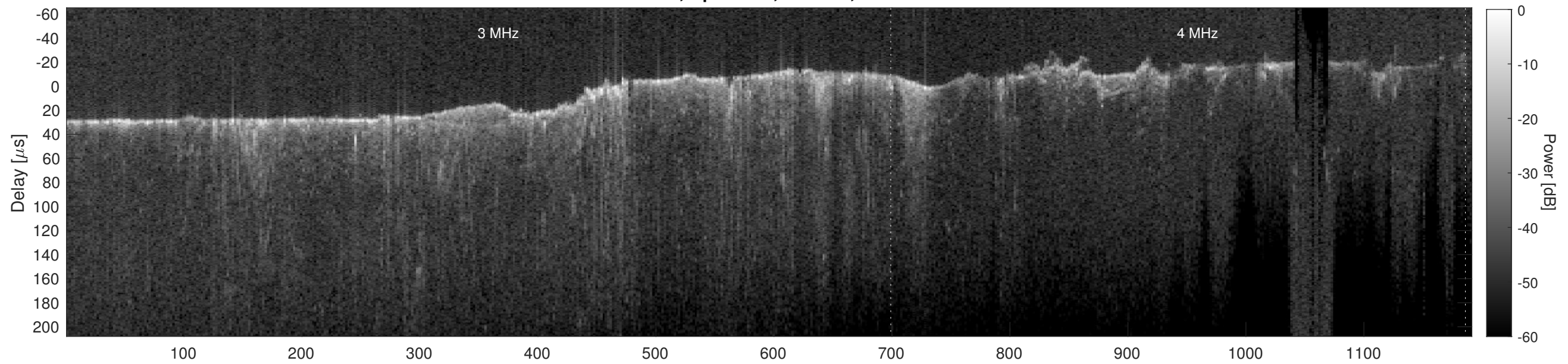
Orbit 7038, Cluttergram
