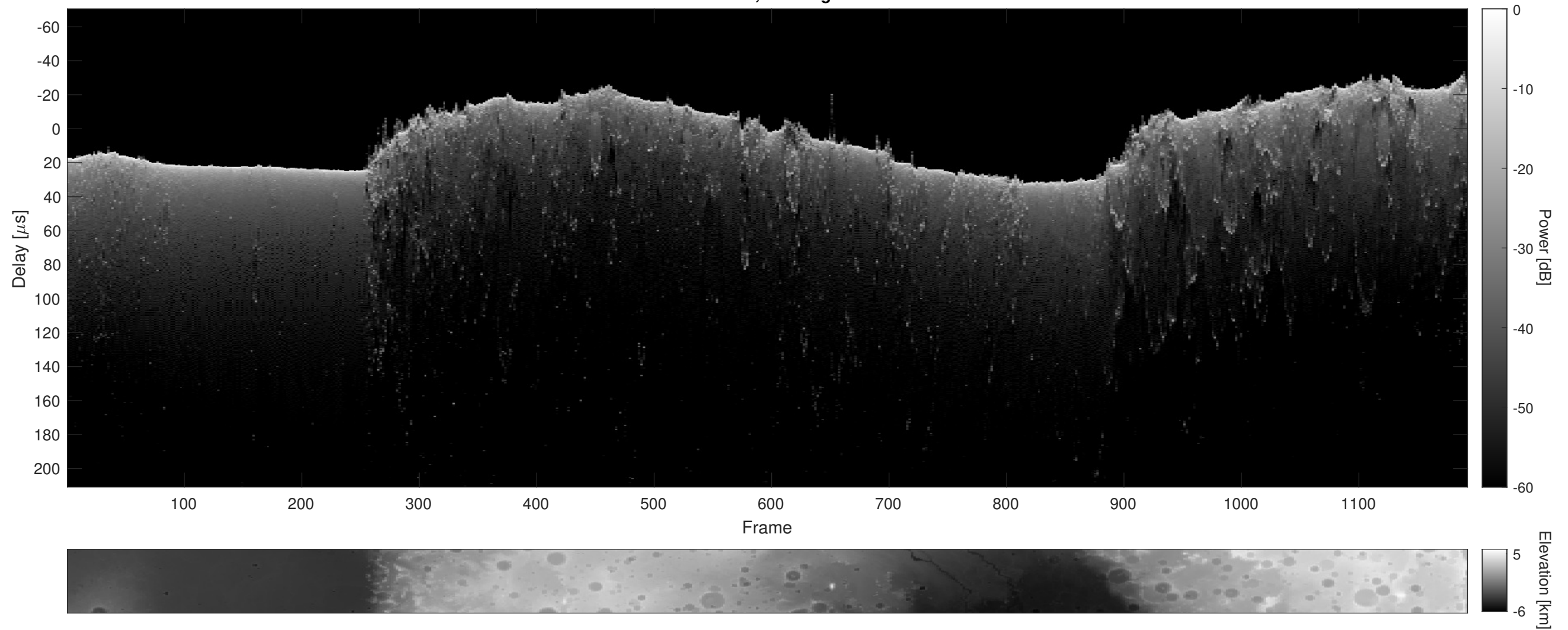
Orbit 7039, Cluttergram
