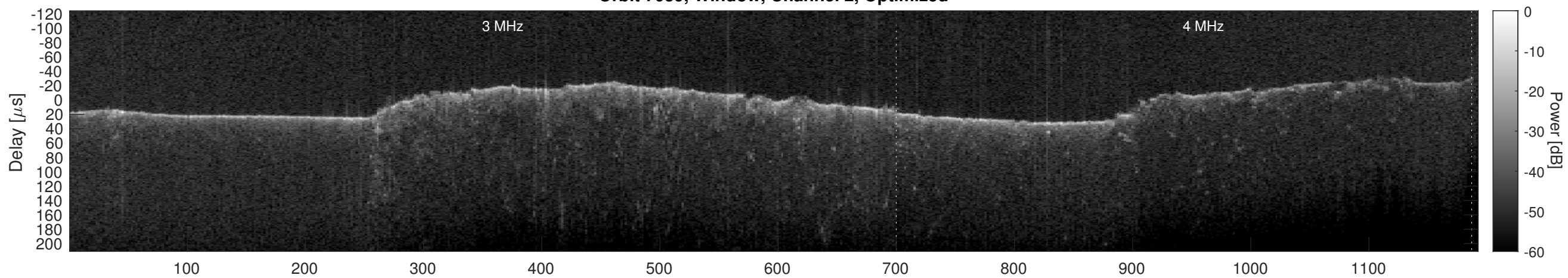
Orbit 7039, Cluttergram
