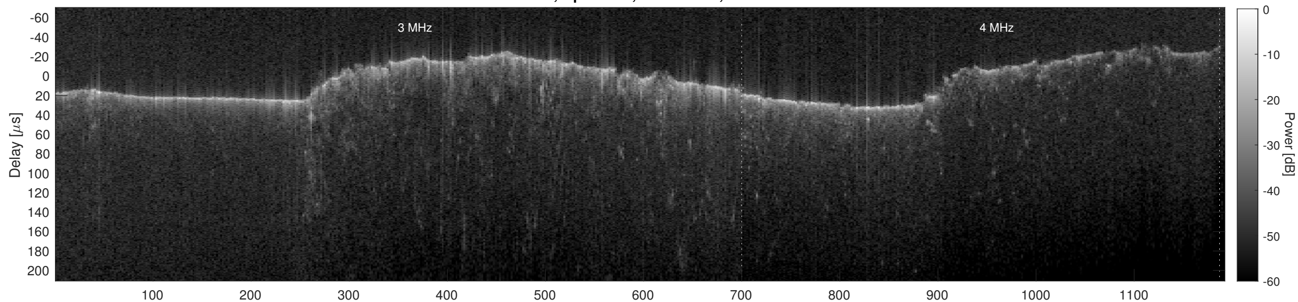
Orbit 7039, Cluttergram
