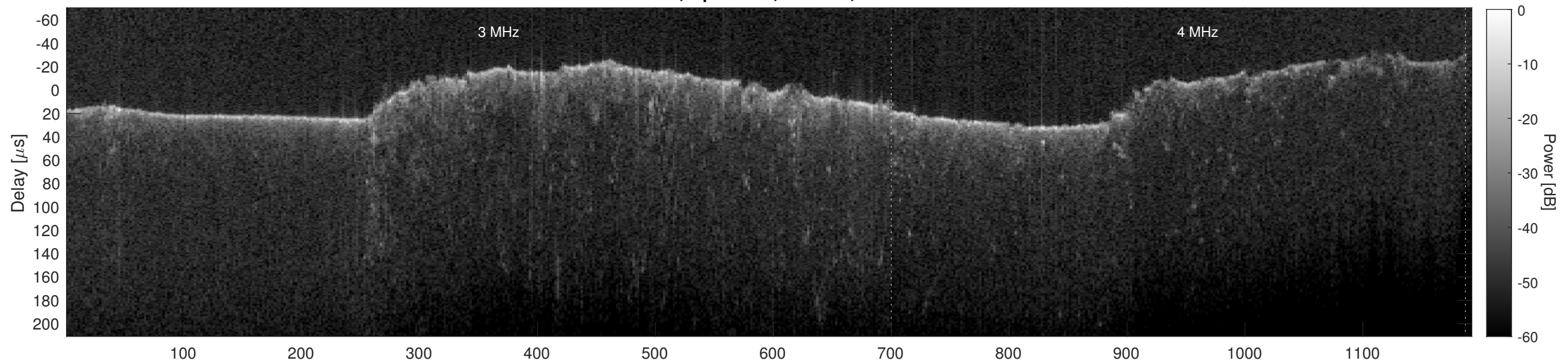
Orbit 7039, Cluttergram
