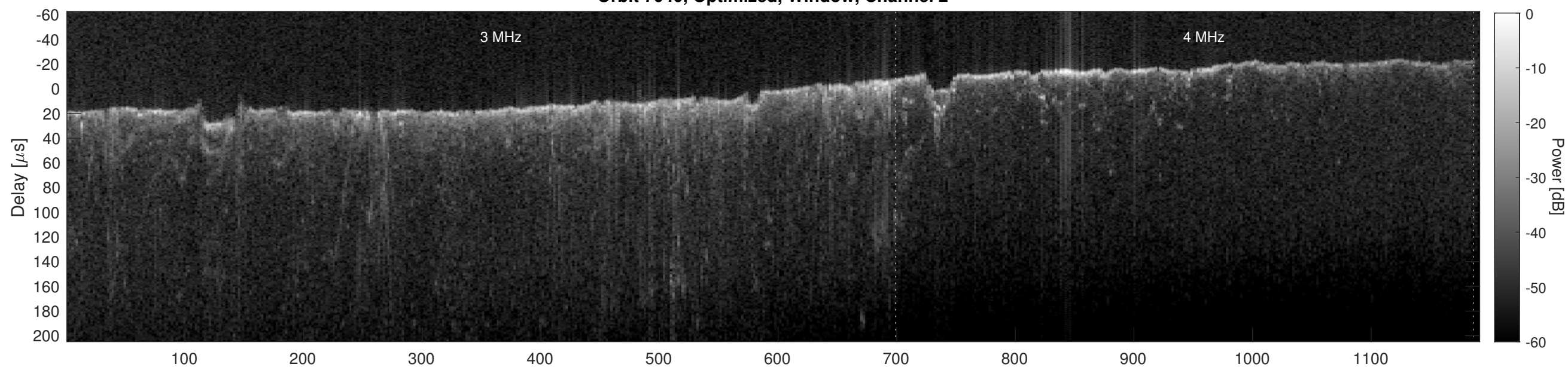
Orbit 7040, Cluttergram
