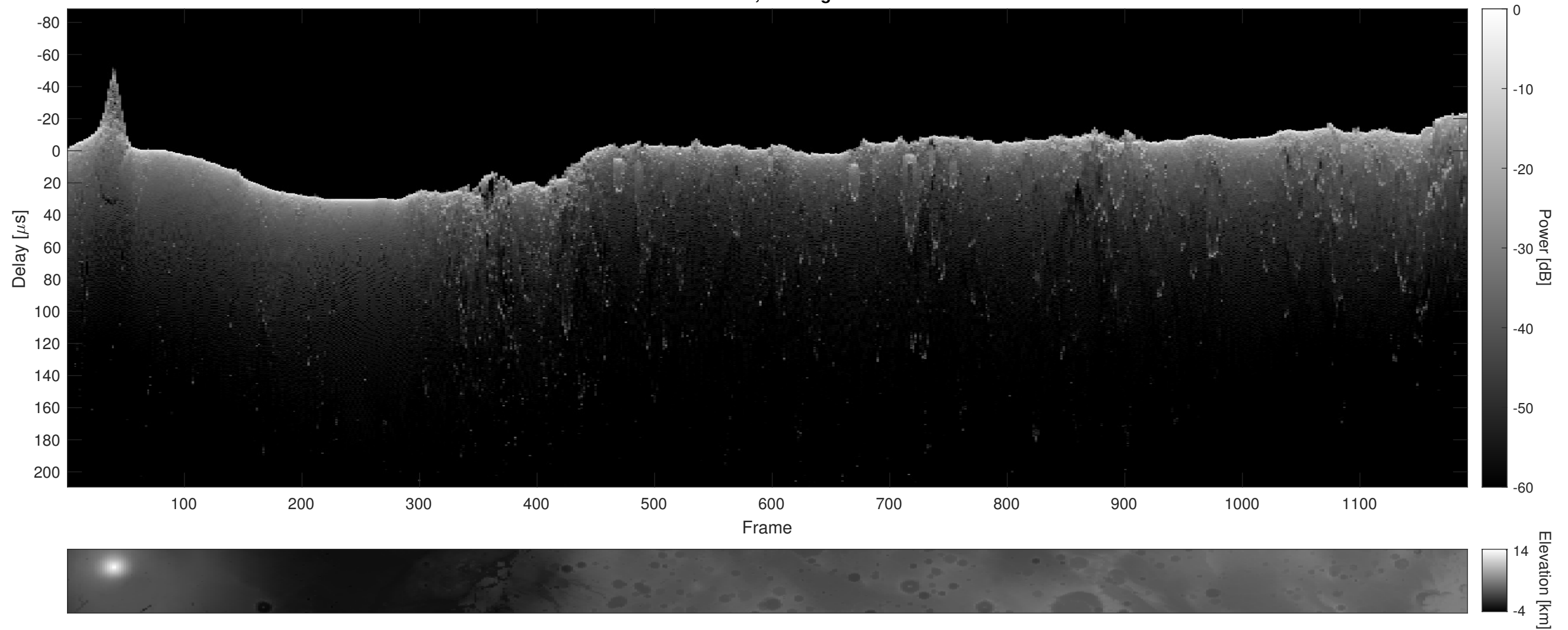
Orbit 7042, Cluttergram
