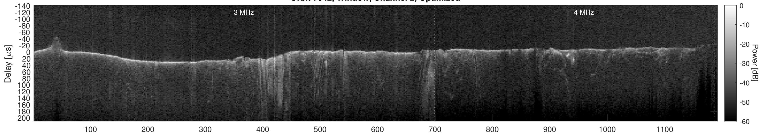
Orbit 7042, Cluttergram
