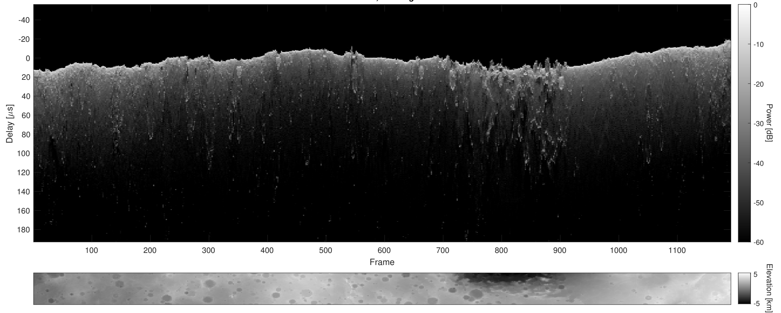
Orbit 7043, Cluttergram
