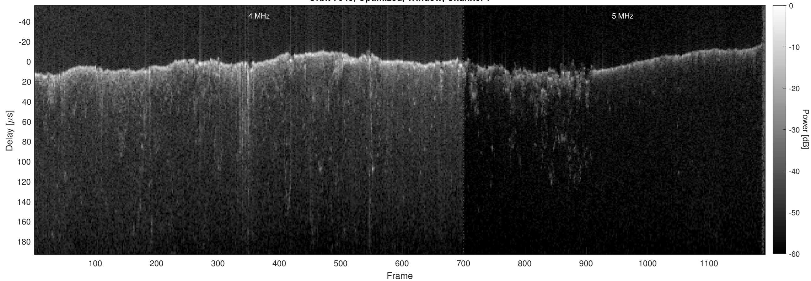
Orbit 7043, Optimized, Window, Channel 2
