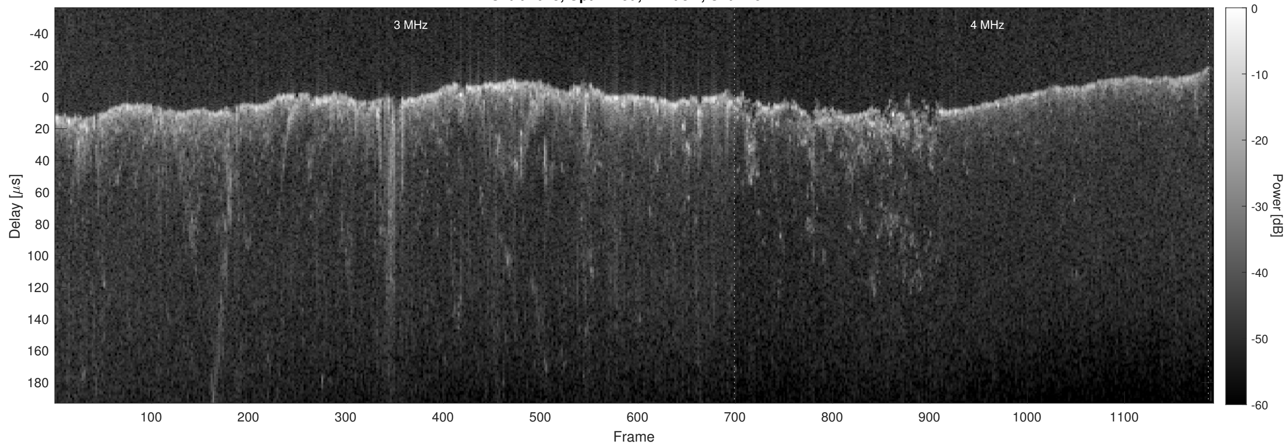
Orbit 7043, Optimized, Window, Channel 2
