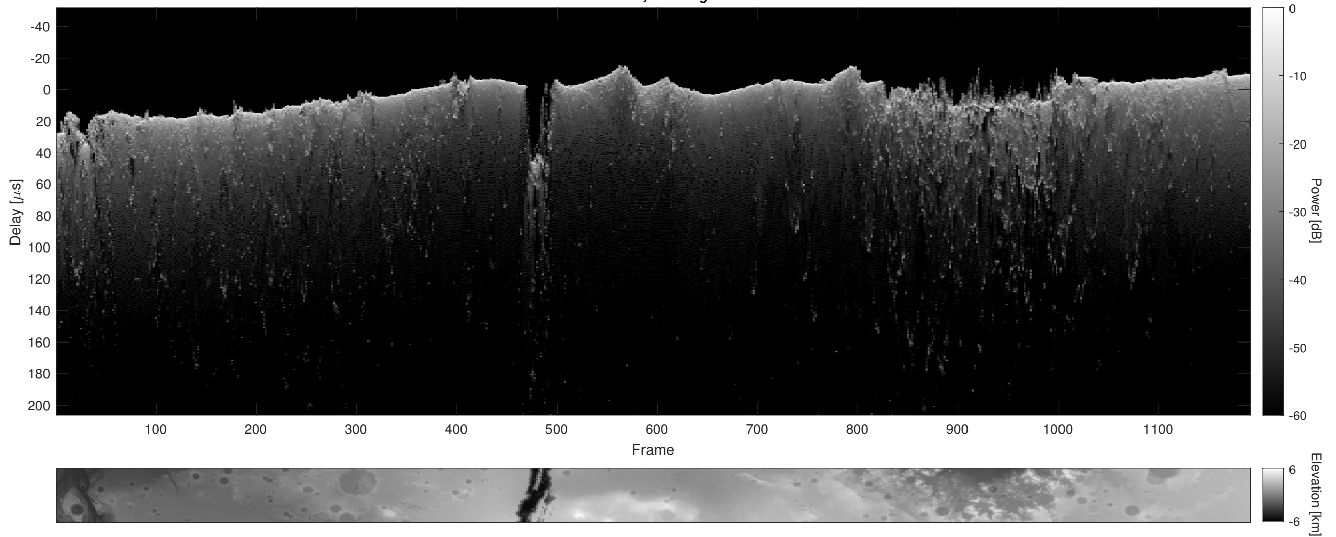
Orbit 7044, Cluttergram
