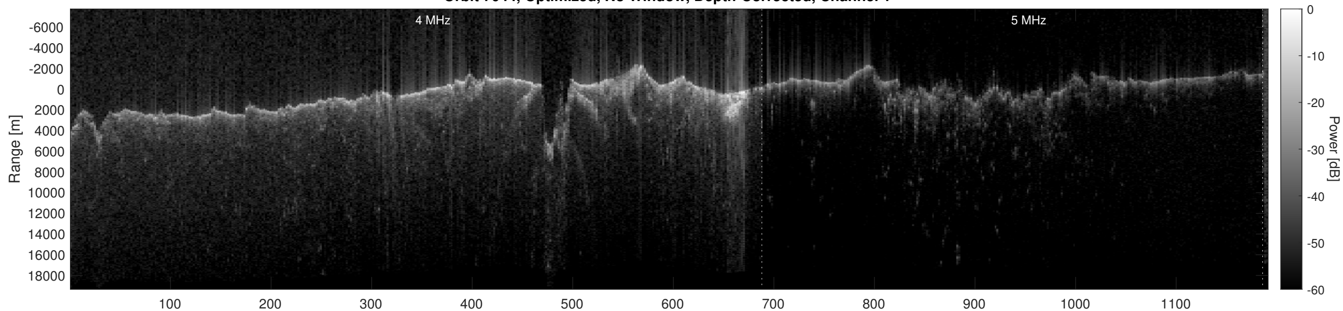
Orbit 7044, Optimized, No Window, Depth-Corrected, Channel 2
