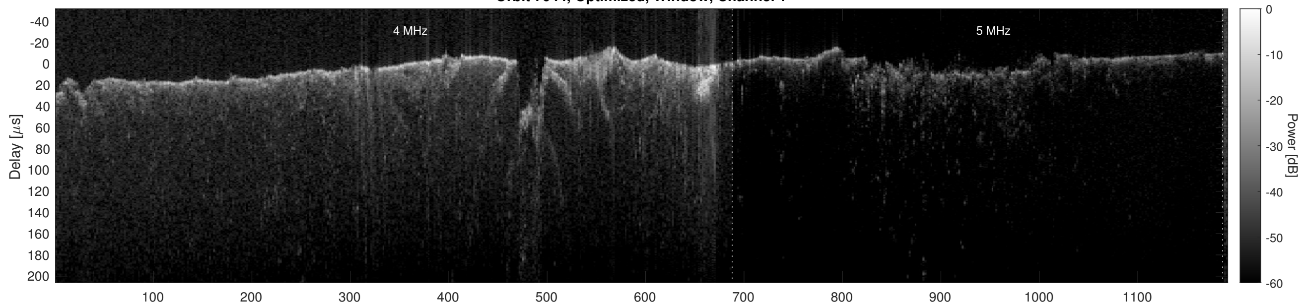
Orbit 7044, Optimized, Window, Channel 2
