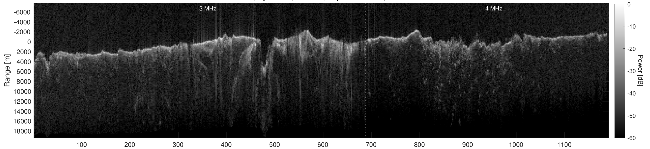
Orbit 7044, Depth-Corrected Cluttergram
