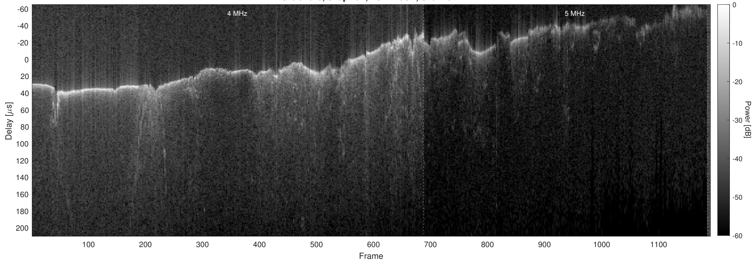
Orbit 7045, Chapman, No Window, Channel 2
