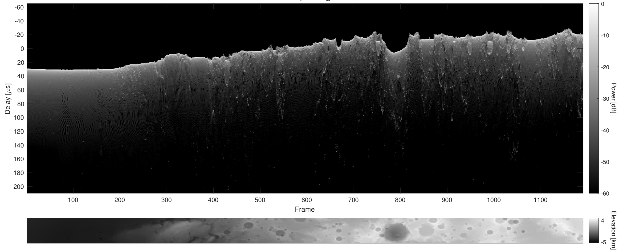
Orbit 7045, Cluttergram
