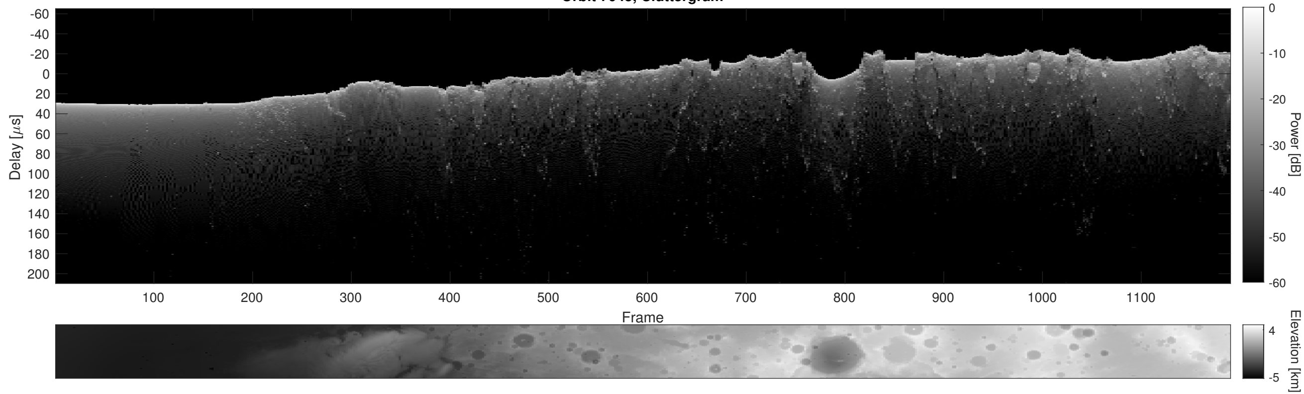
Orbit 7045, Cluttergram
