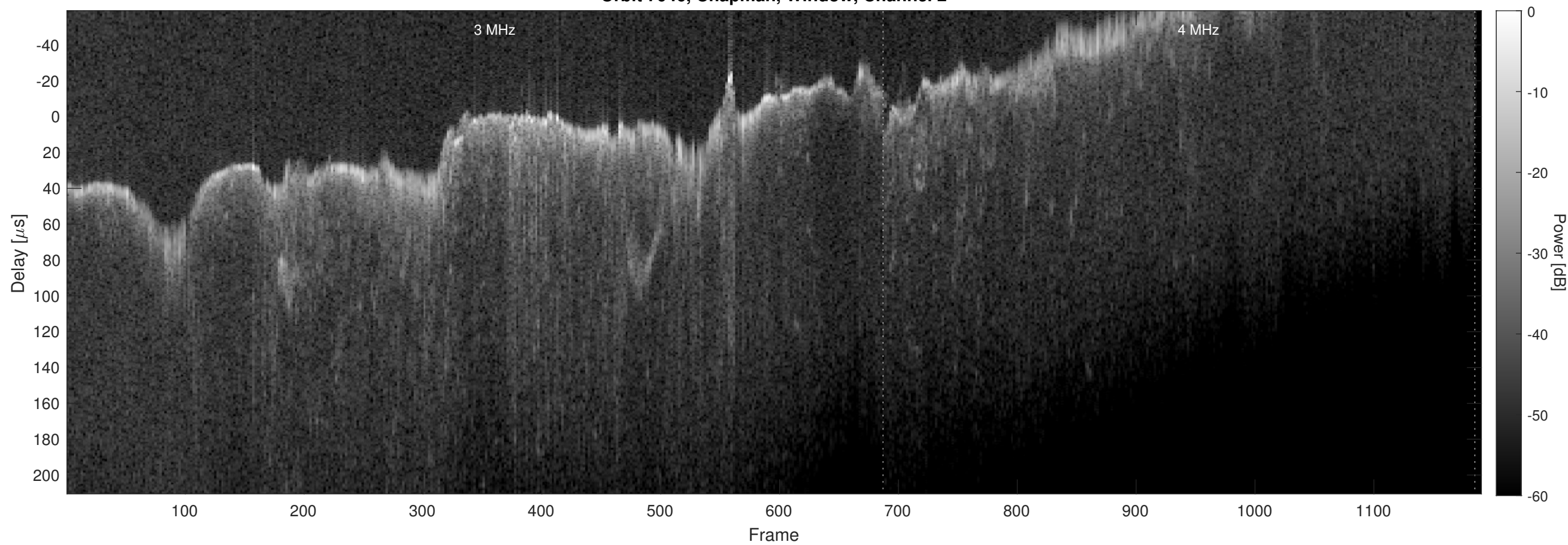
Orbit 7046, Chapman, Window, Channel 2
