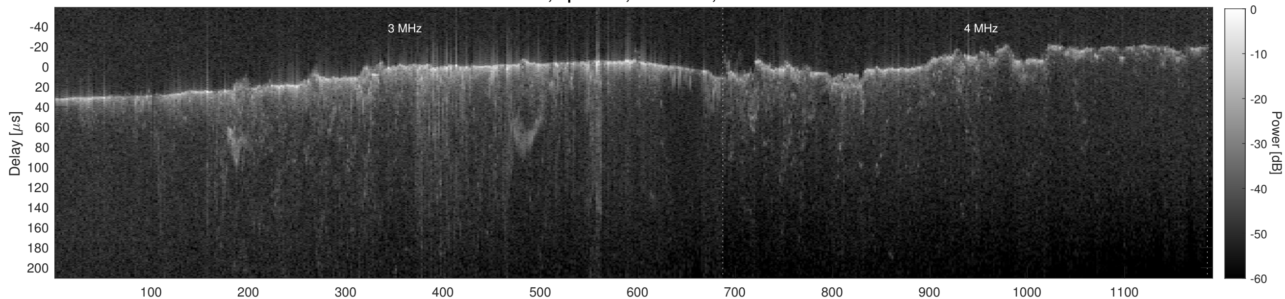
Orbit 7046, Cluttergram
