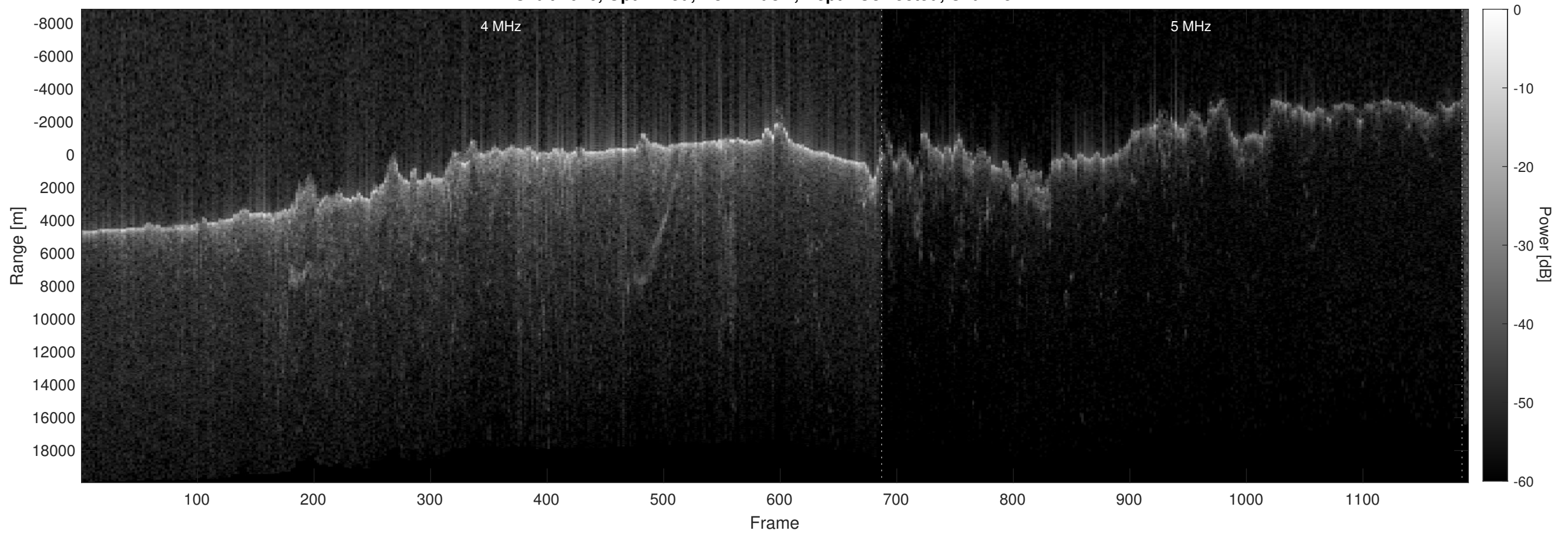
Orbit 7046, Optimized, No Window, Depth-Corrected, Channel 2
