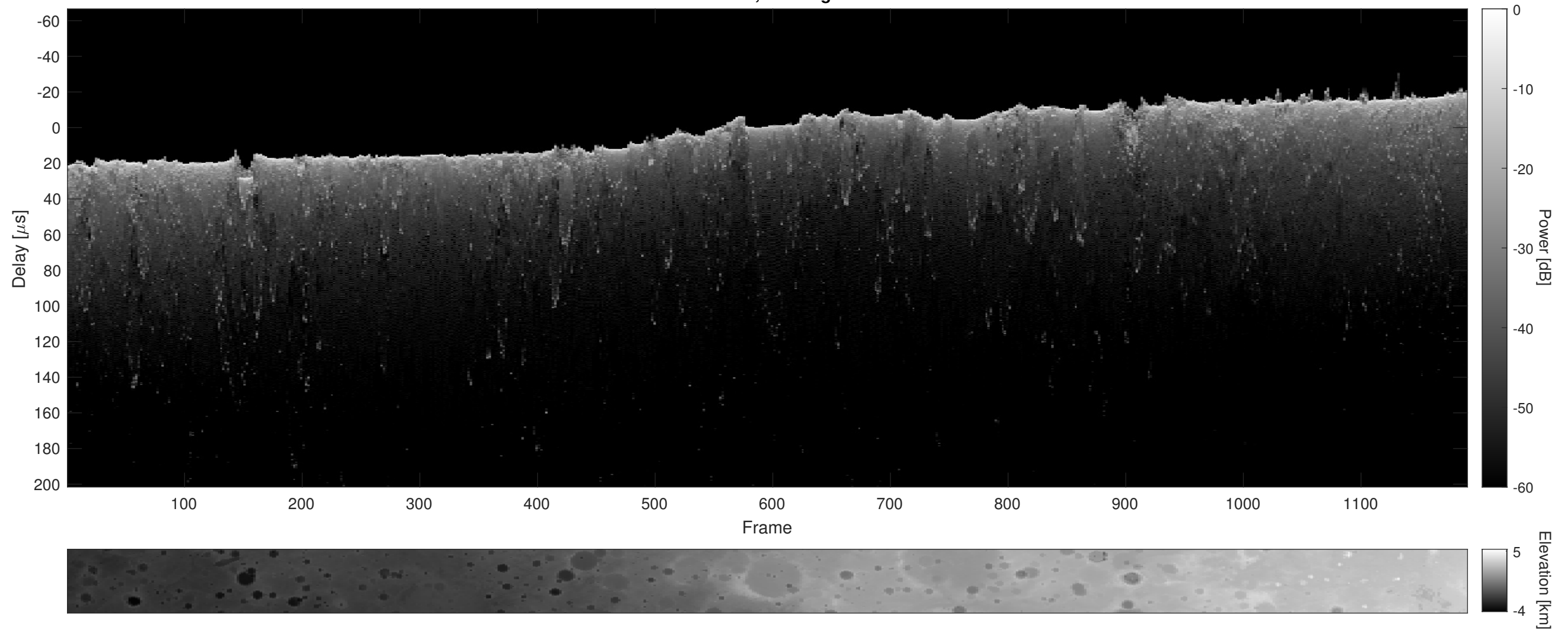
Orbit 7047, Cluttergram
