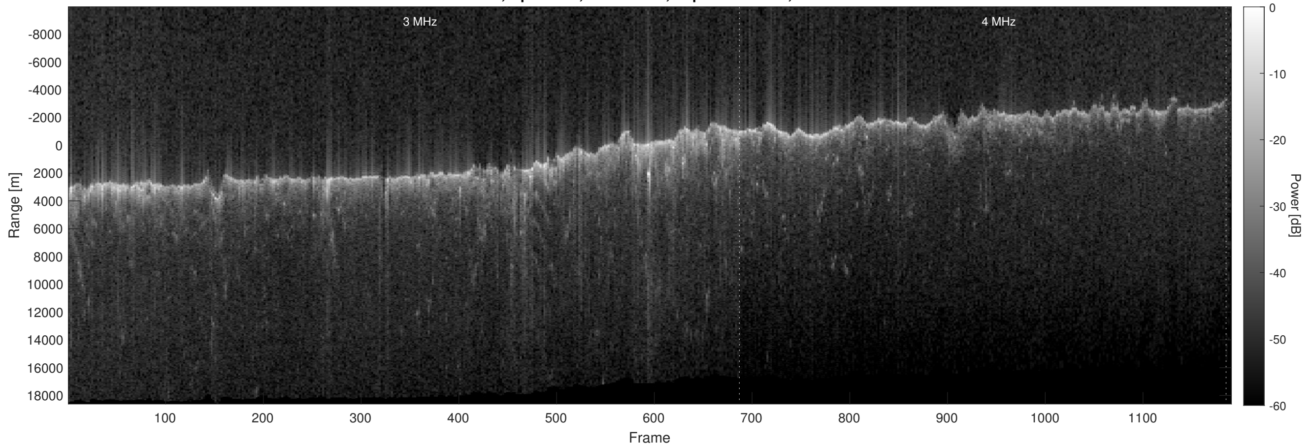
Orbit 7047, Optimized, No Window, Depth-Corrected, Channel 2
