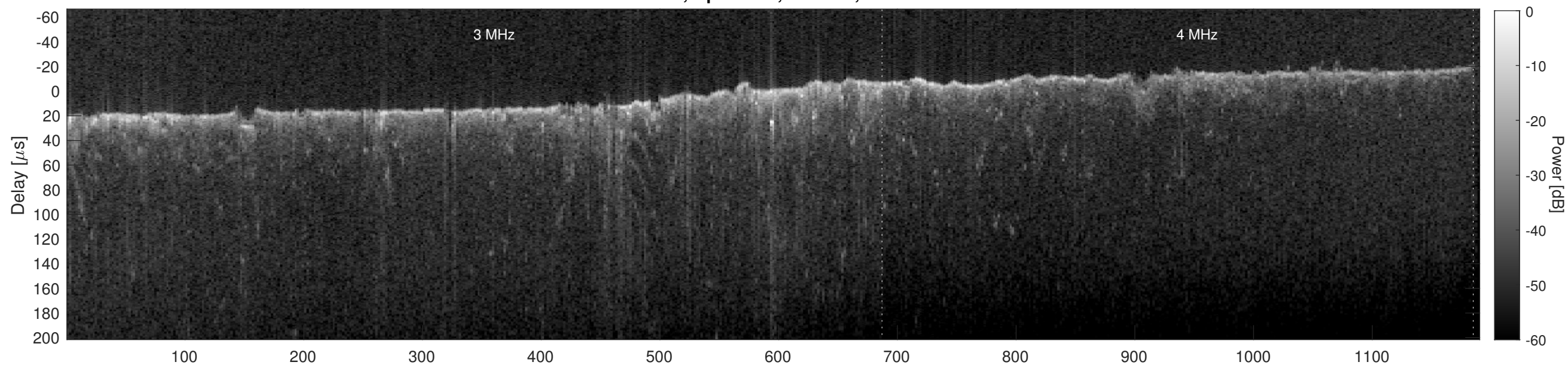
Orbit 7047, Cluttergram
