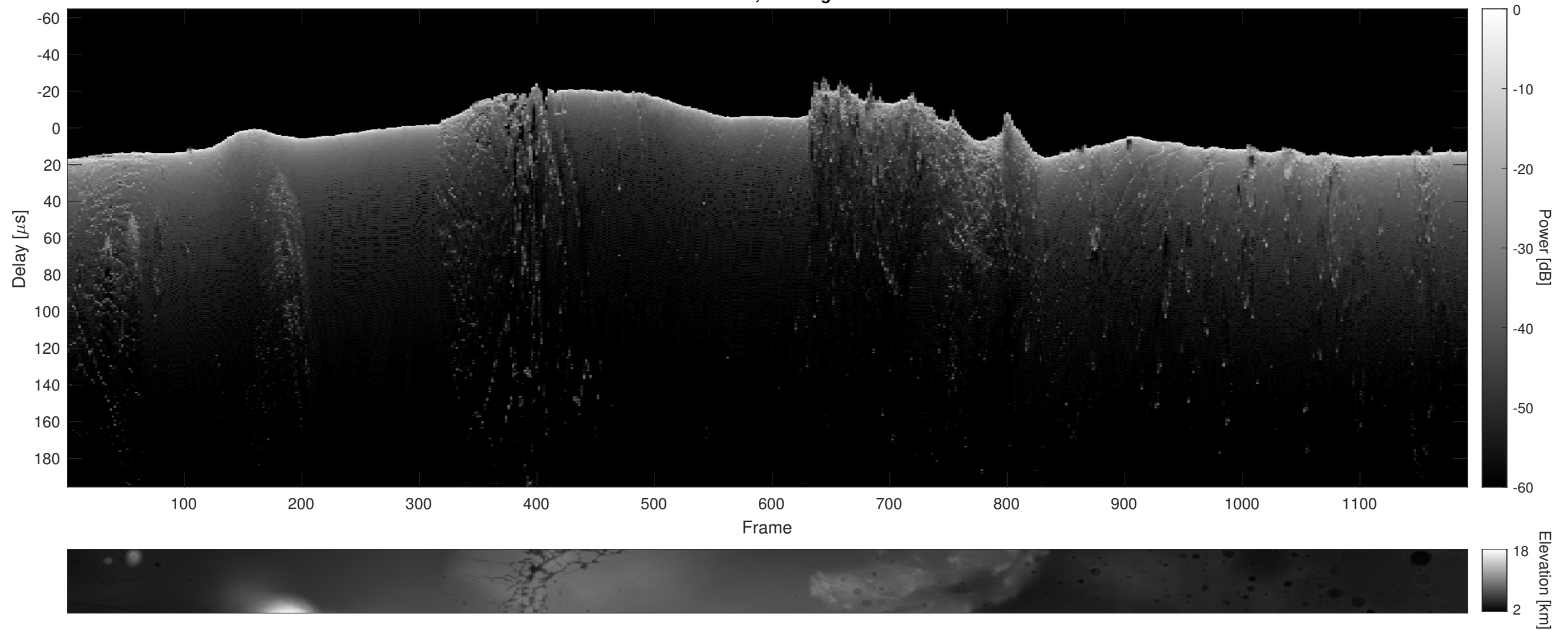
Orbit 7048, Cluttergram
