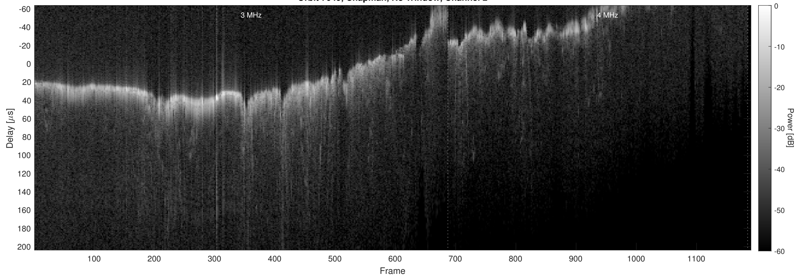
Orbit 7049, Chapman, No Window, Channel 2
