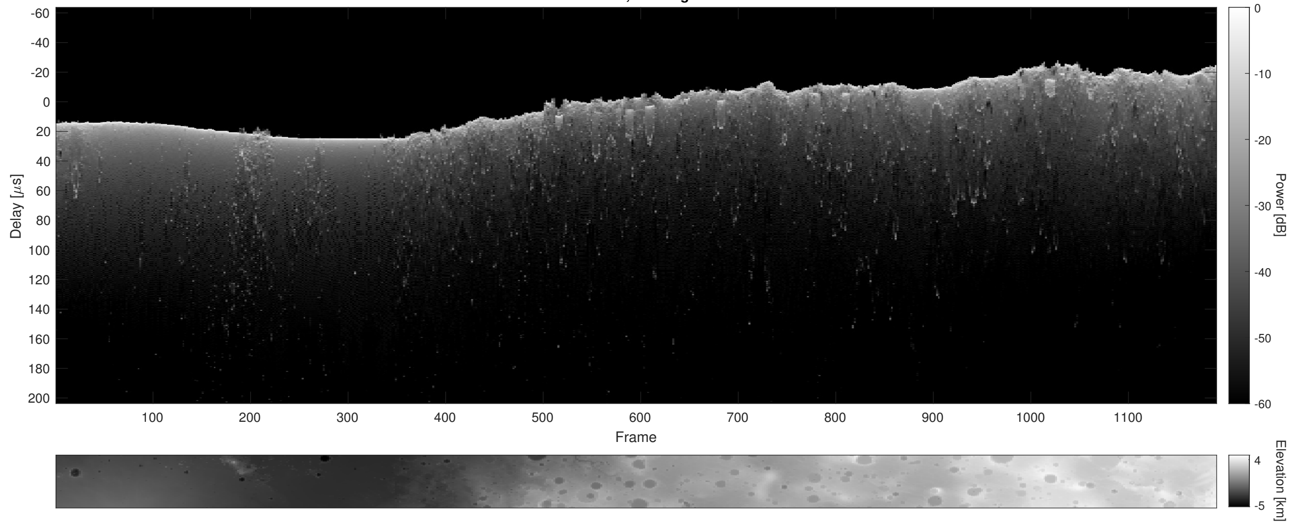
Orbit 7049, Cluttergram
