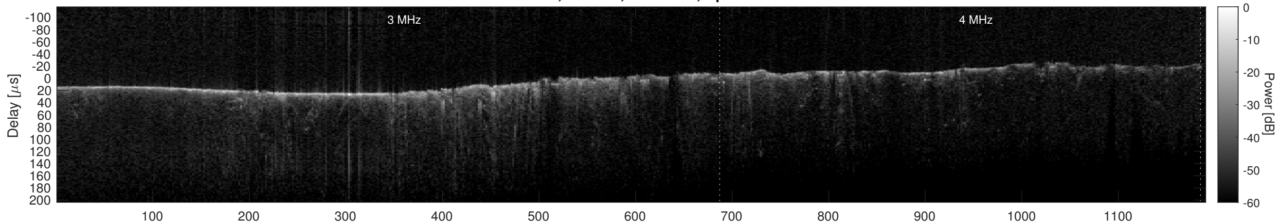
Orbit 7049, Cluttergram
