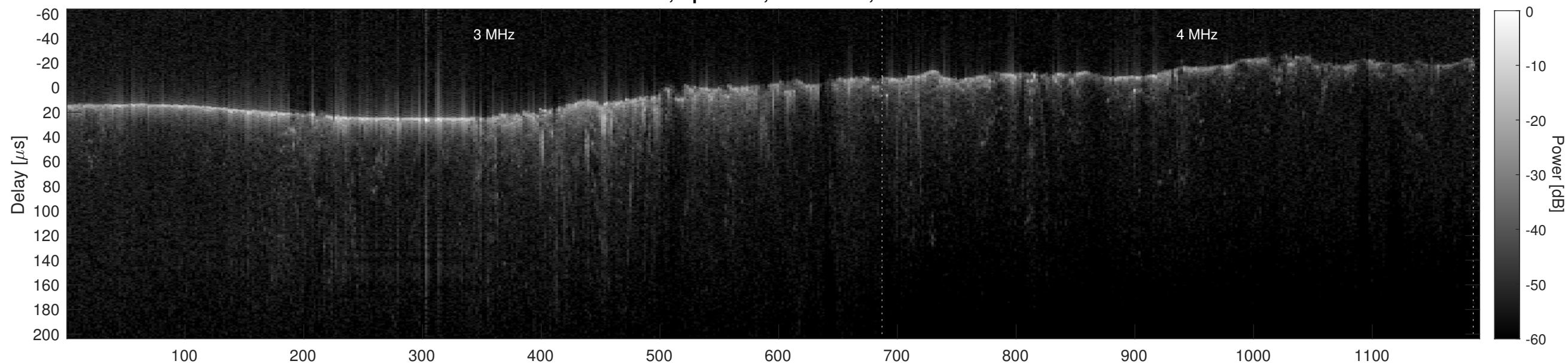
Orbit 7049, Cluttergram
