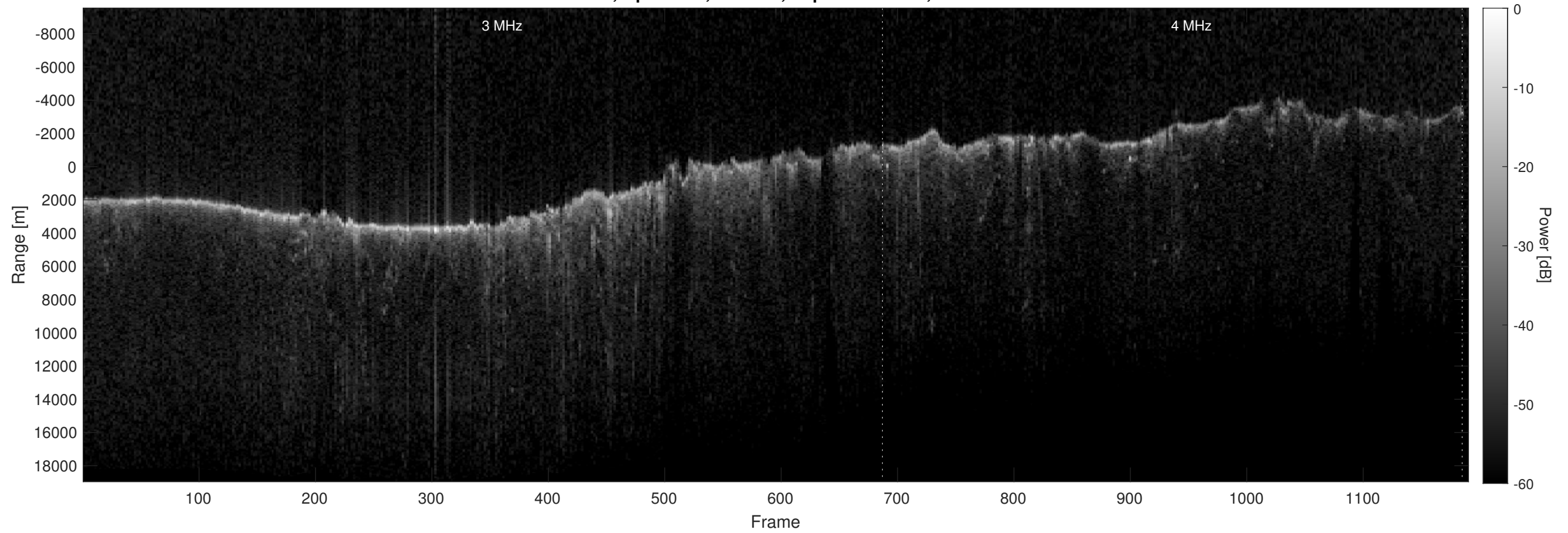
Orbit 7049, Optimized, Window, Depth-Corrected, Channel 2
