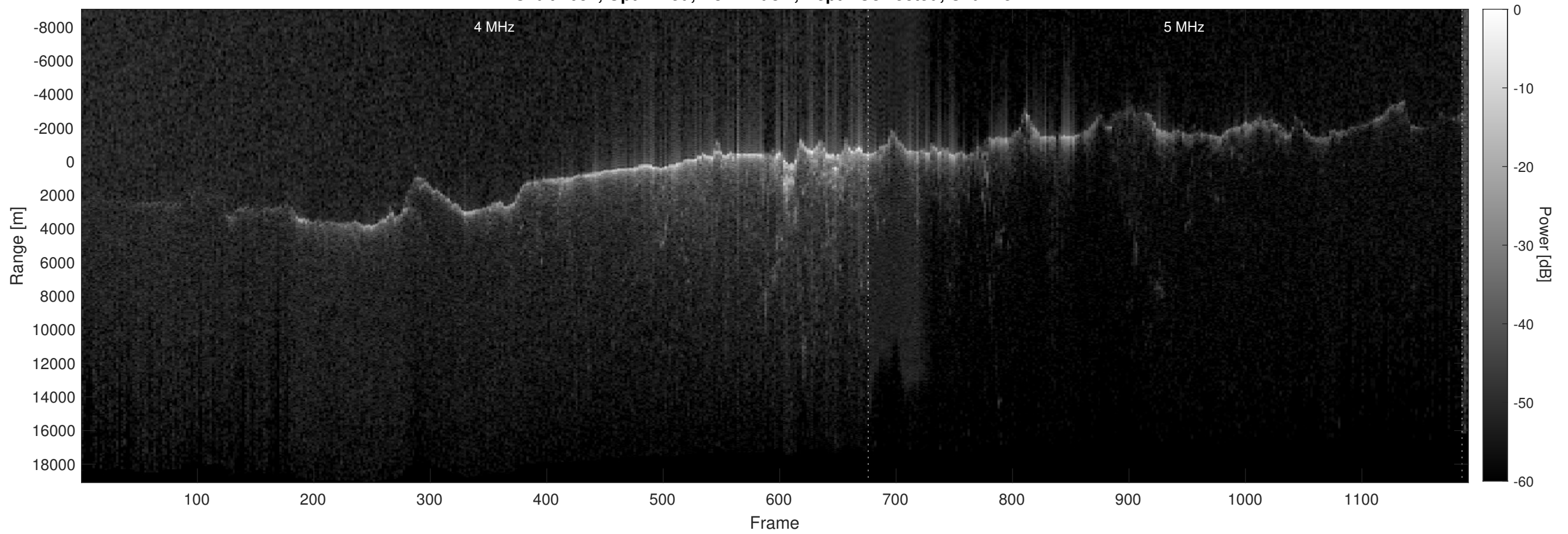
Orbit 7052, Optimized, No Window, Depth-Corrected, Channel 2
