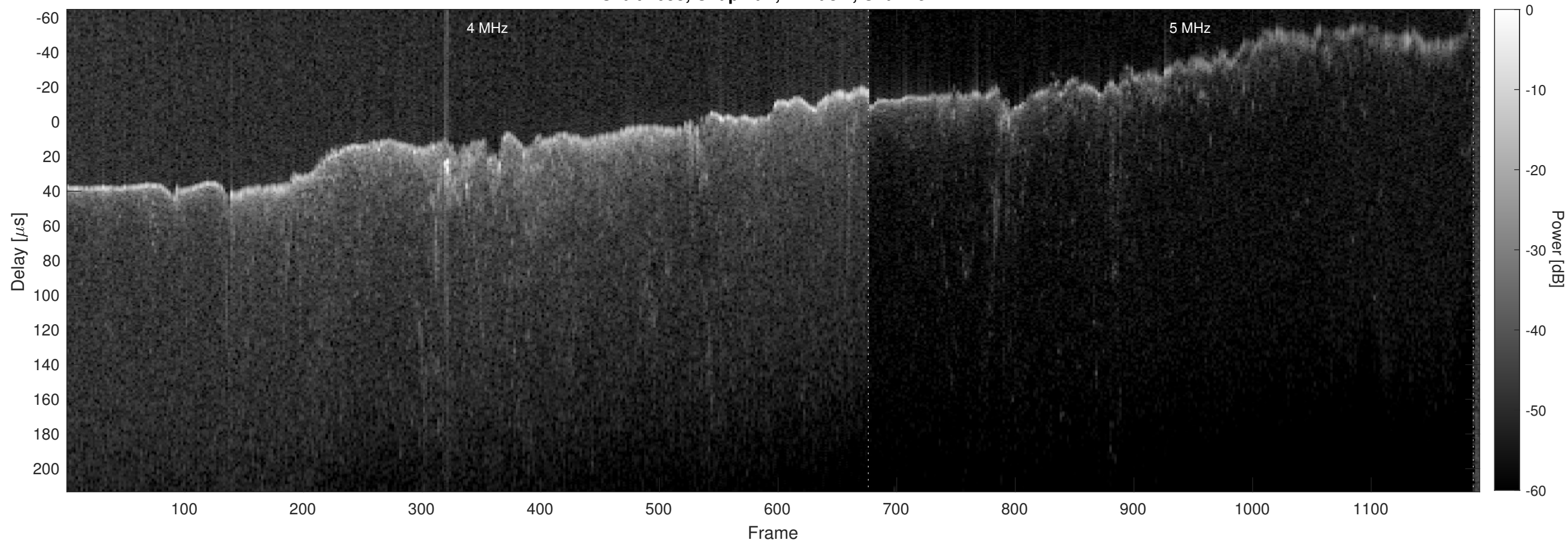
Orbit 7053, Chapman, Window, Channel 2
