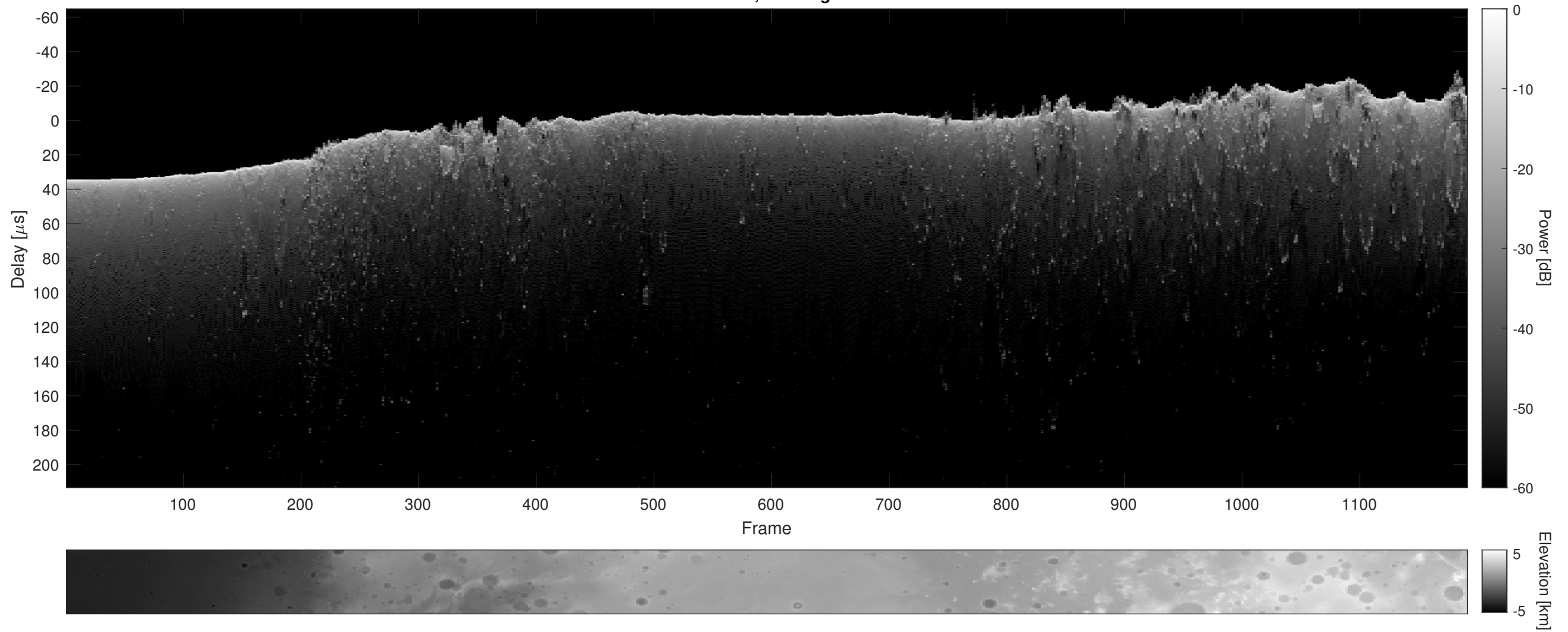
Orbit 7053, Cluttergram
