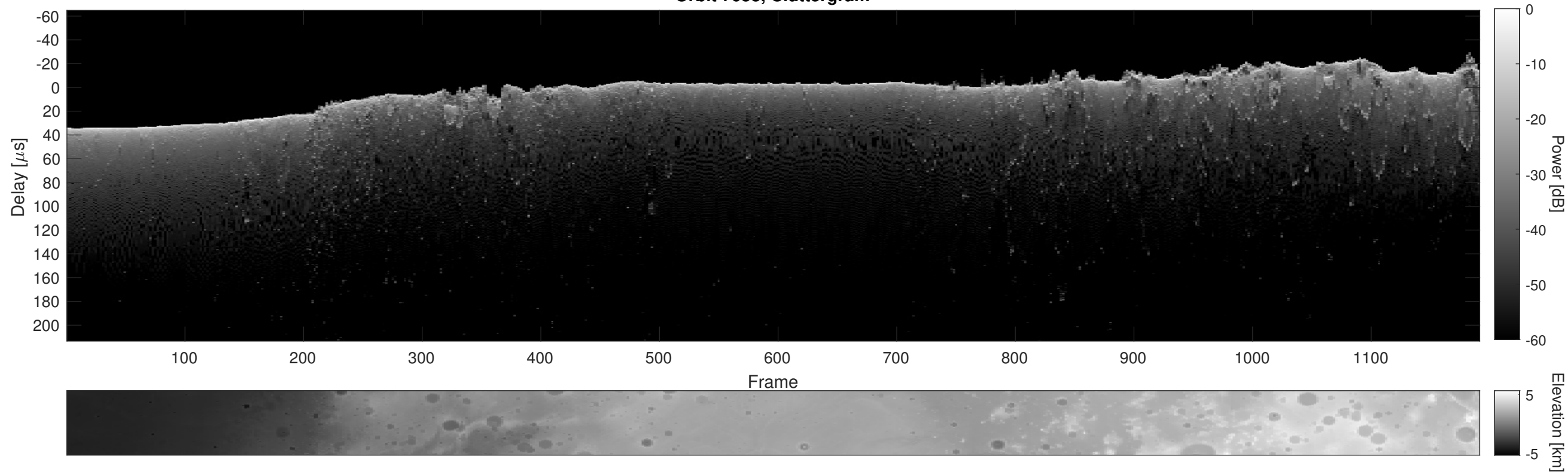
Orbit 7053, Cluttergram
