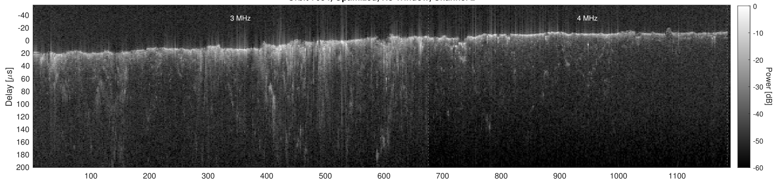
Orbit 7054, Cluttergram
