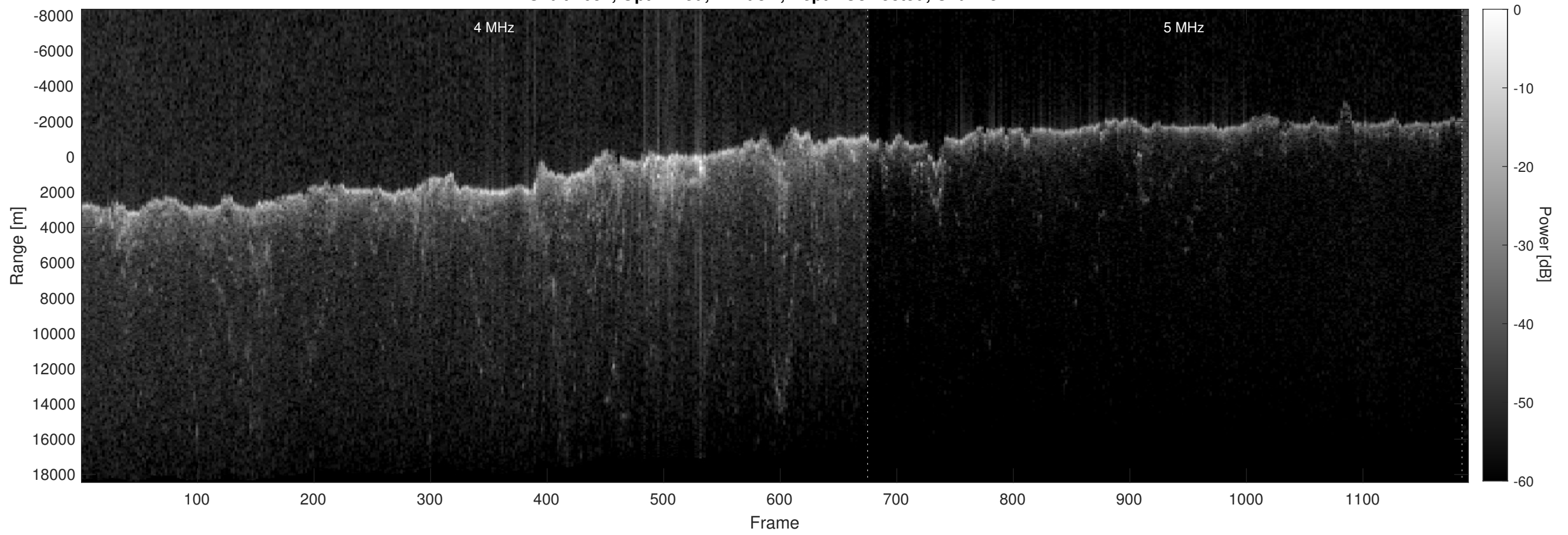
Orbit 7054, Optimized, Window, Depth-Corrected, Channel 2
