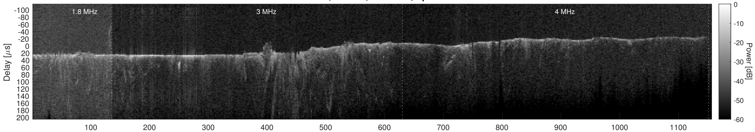
Orbit 7056, Cluttergram
