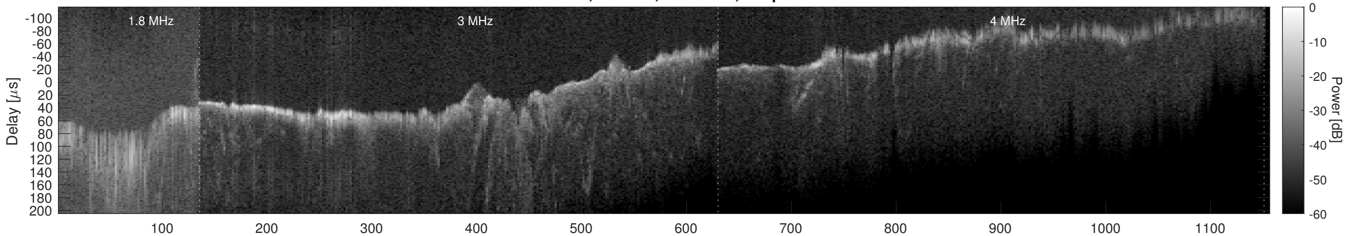
Orbit 7056, Window, Channel 2, Optimized
