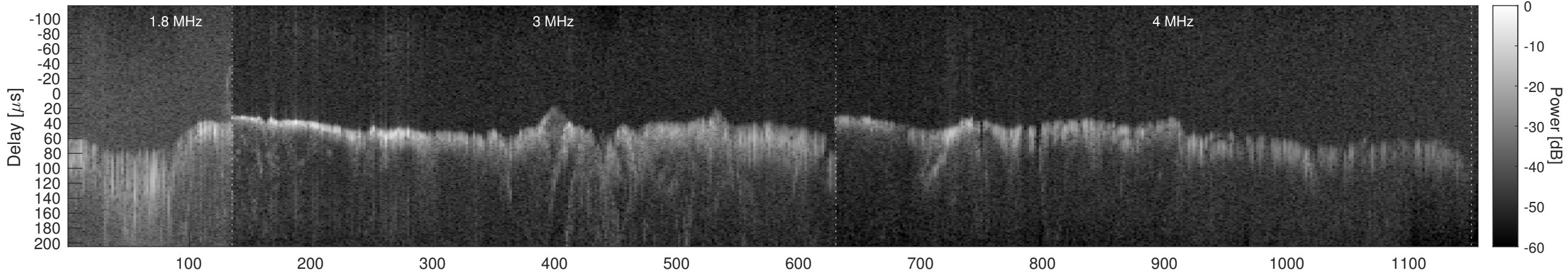
Orbit 7056, Window, Channel 2, Chapman
