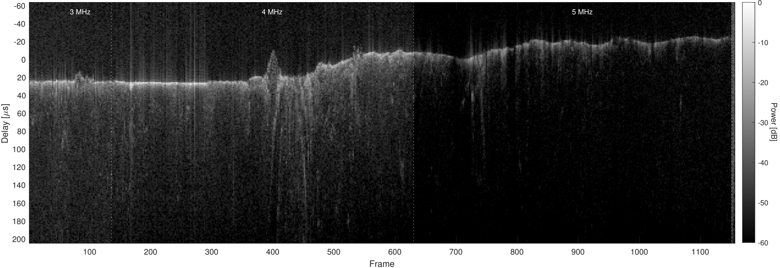
Orbit 7056, Optimized, No Window, Channel 2
