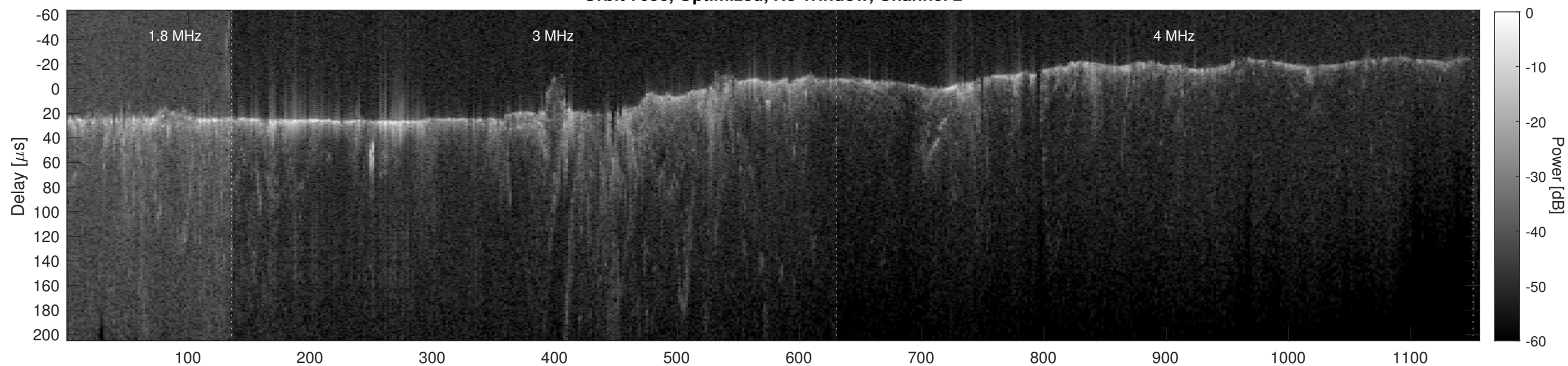
Orbit 7056, Cluttergram
