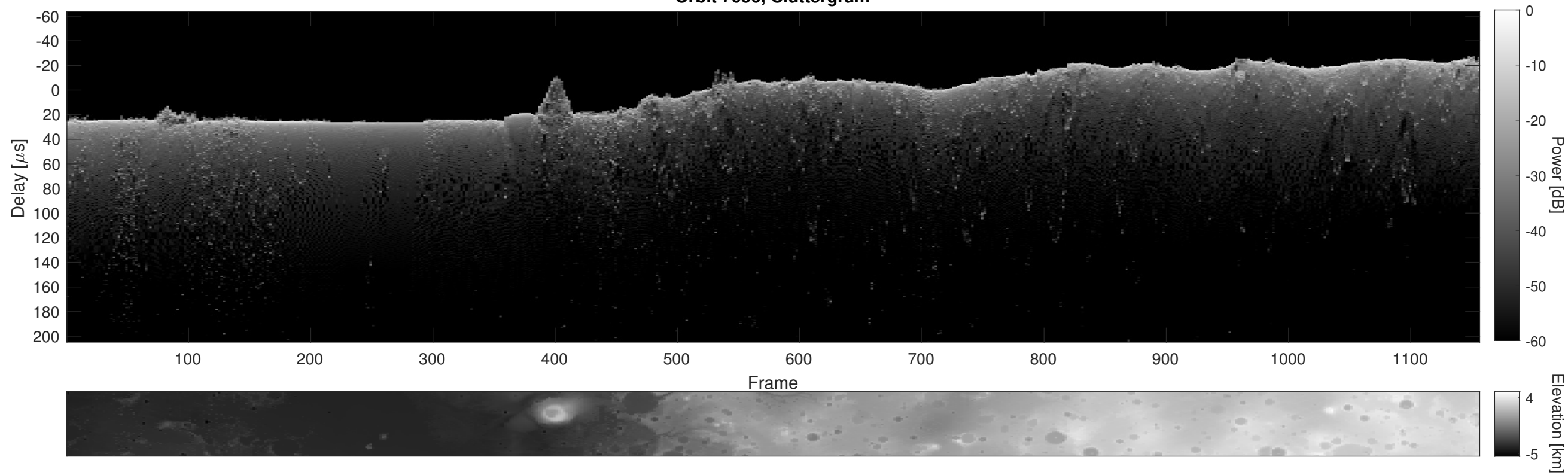
Orbit 7056, Cluttergram
