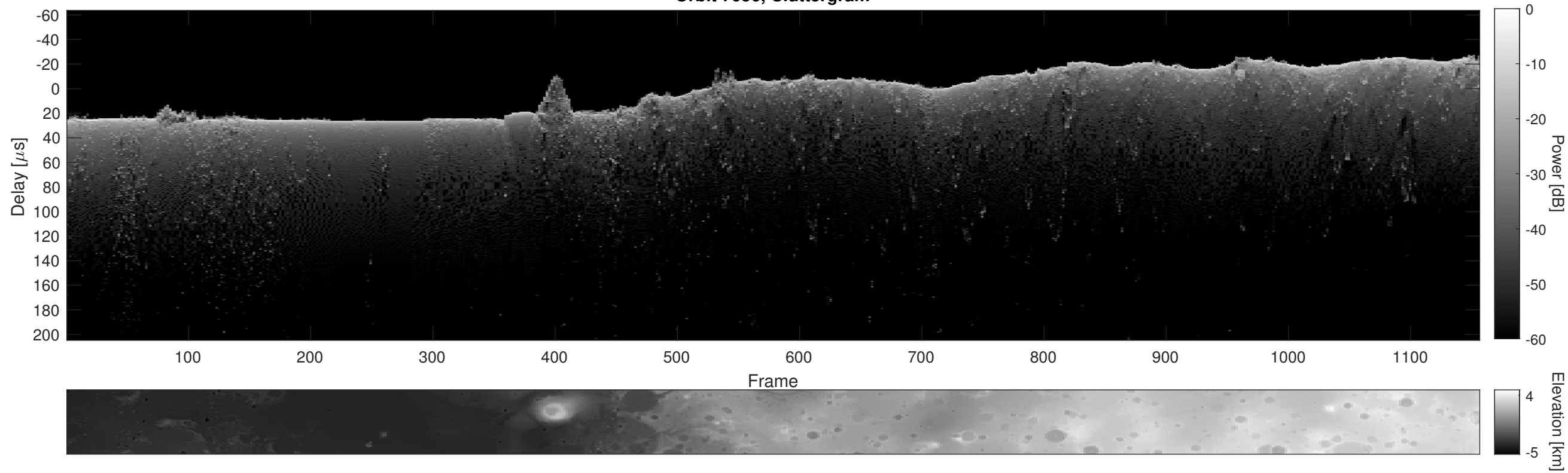
Orbit 7056, Cluttergram
