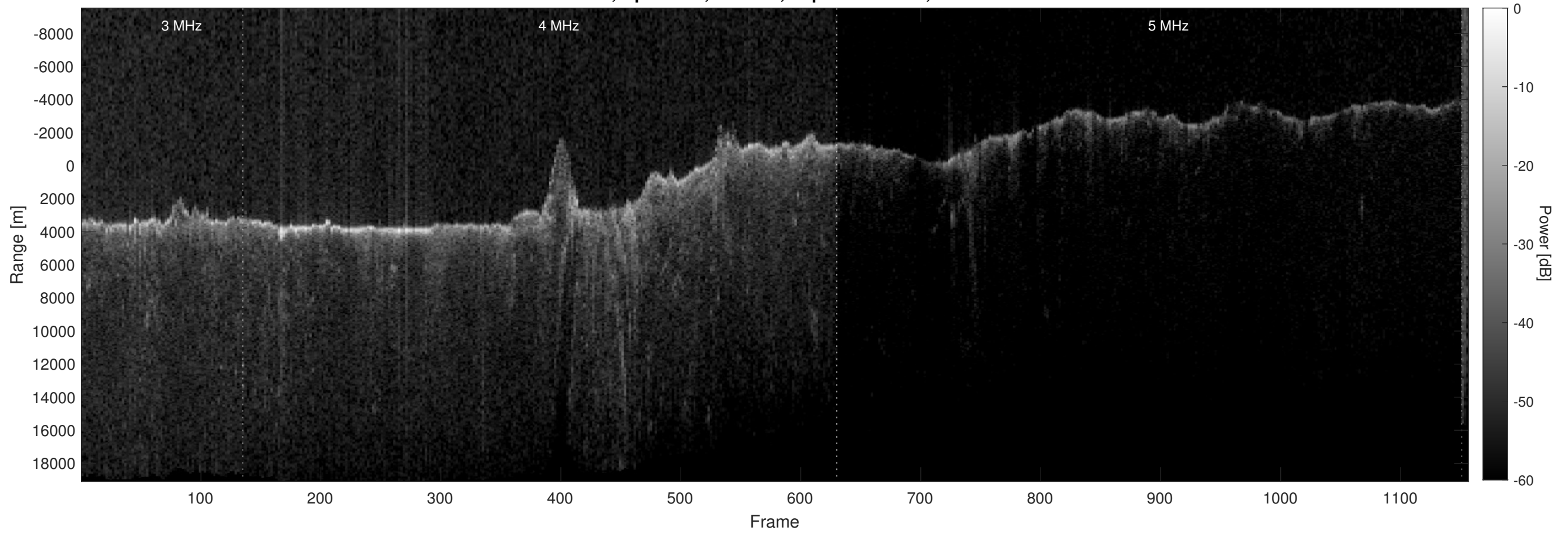
Orbit 7056, Optimized, Window, Depth-Corrected, Channel 2
