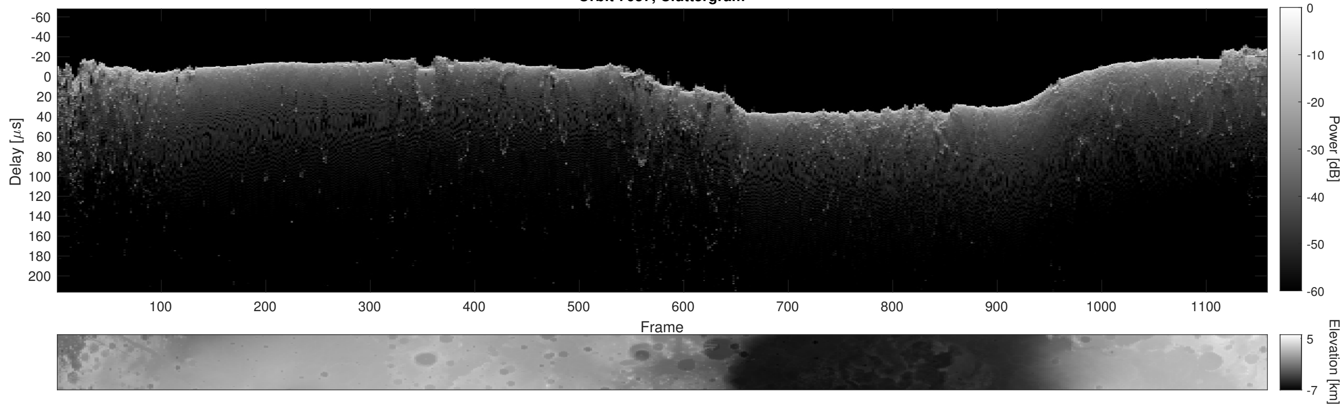
Orbit 7057, Cluttergram
